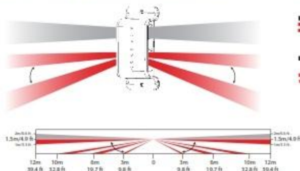
Figure 1: Vertical Beam Adjustment (Lower Only)
